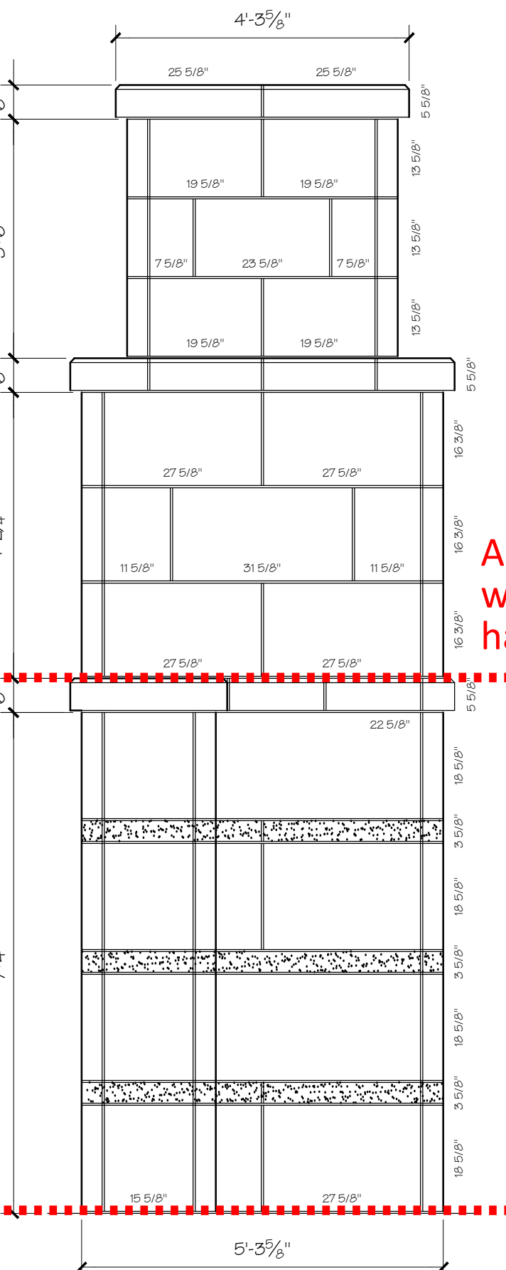
3 SIDE VIEW @ TOWER 1/2" = 1'-0"
