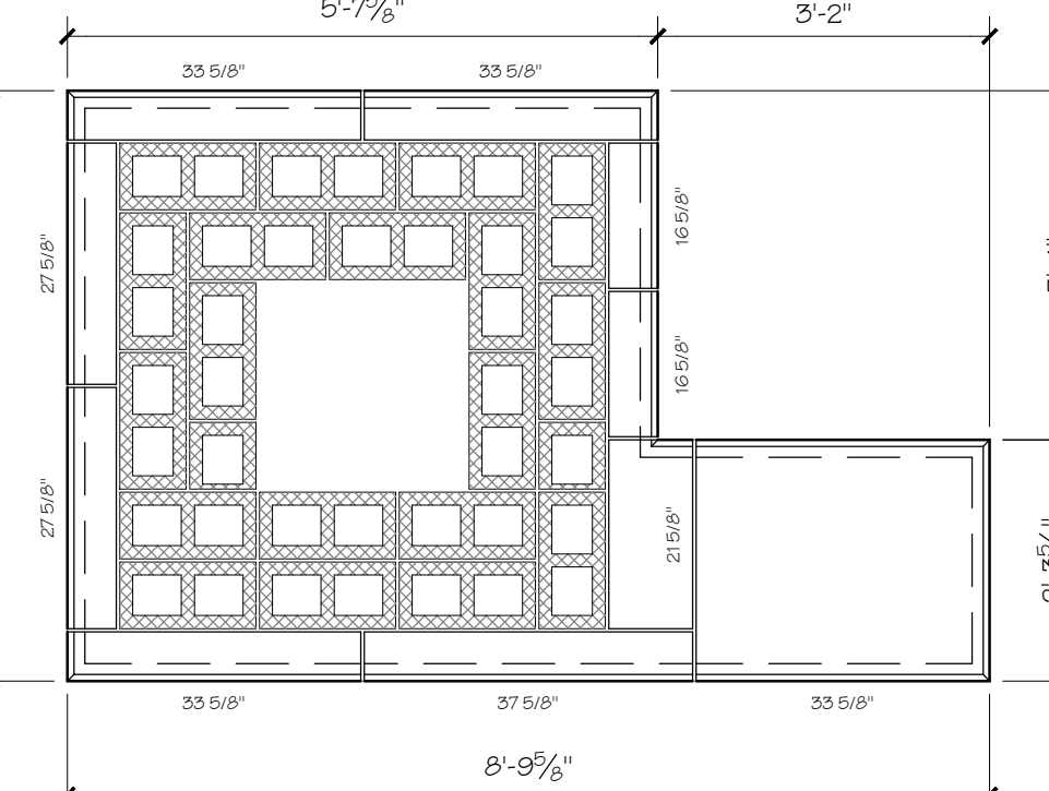
8 PLAN VIEW @ TOWER CAP 1/2" = 1'-0"
