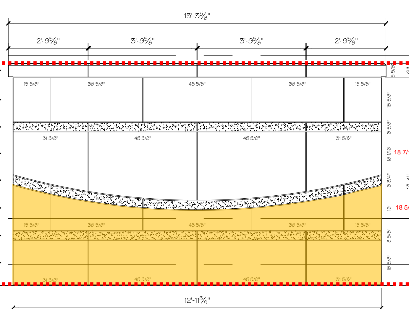
4 ELEVATION @ WALL 1/2" = 1'-0"
