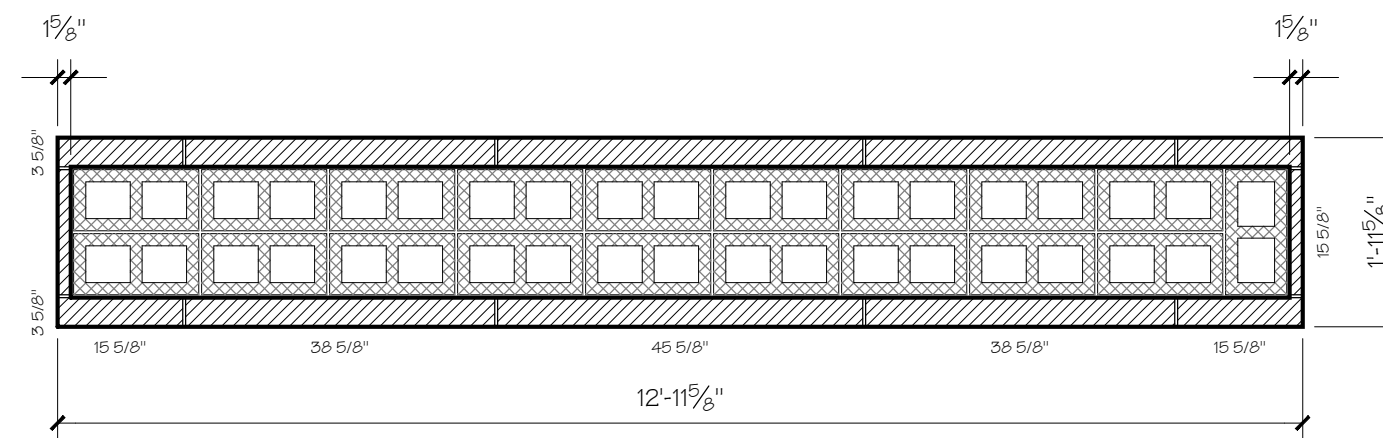
16 ELEVATION @ WALL 1/2" = 1'-0"
