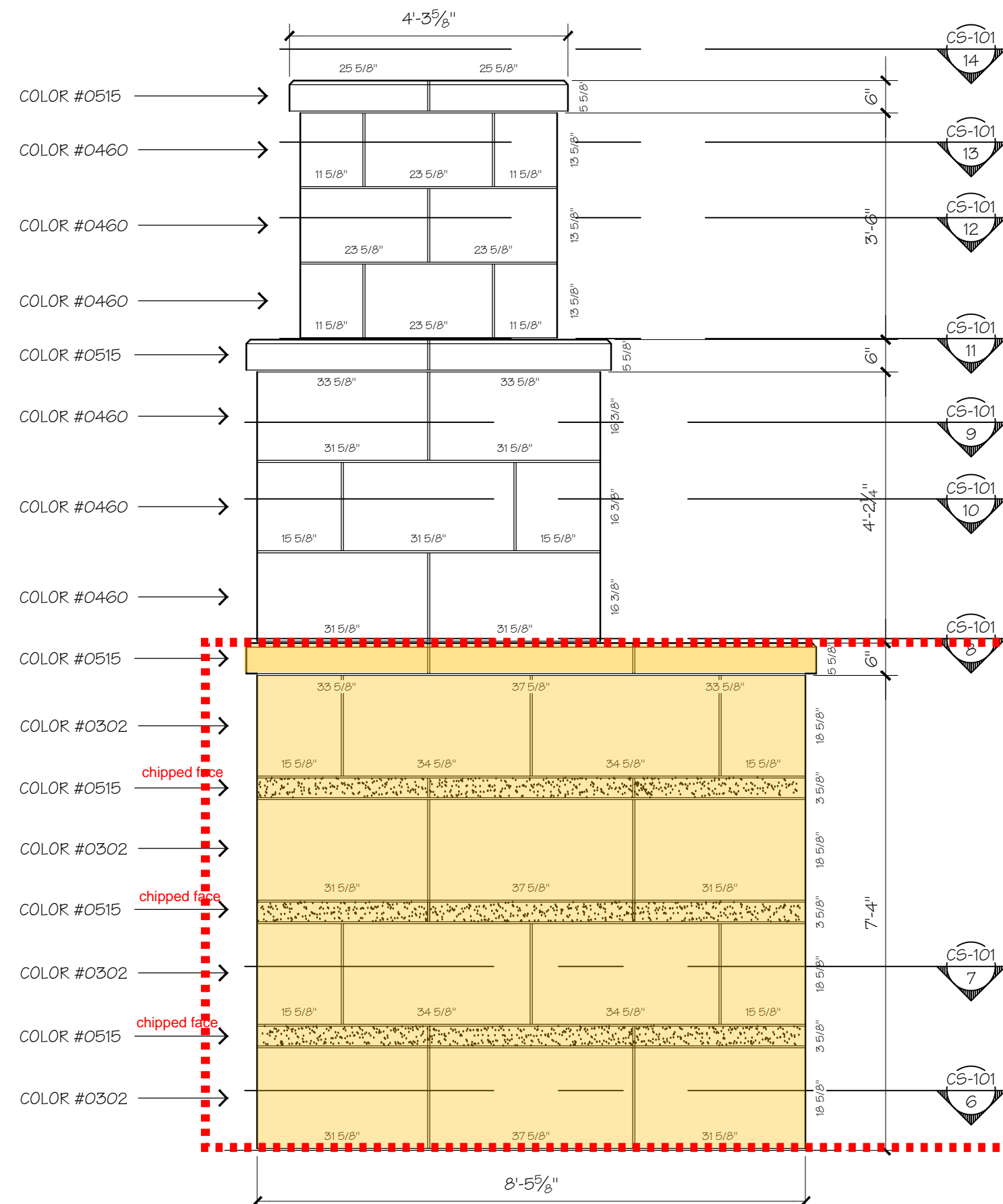
2 ELEVATION @ TOWER 1/2" = 1'-0"
