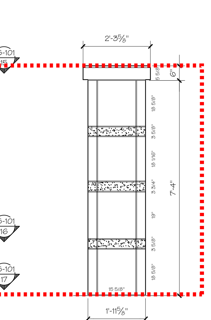
5 SIDE VIEW @ WALL 1/2" = 1'-0"
