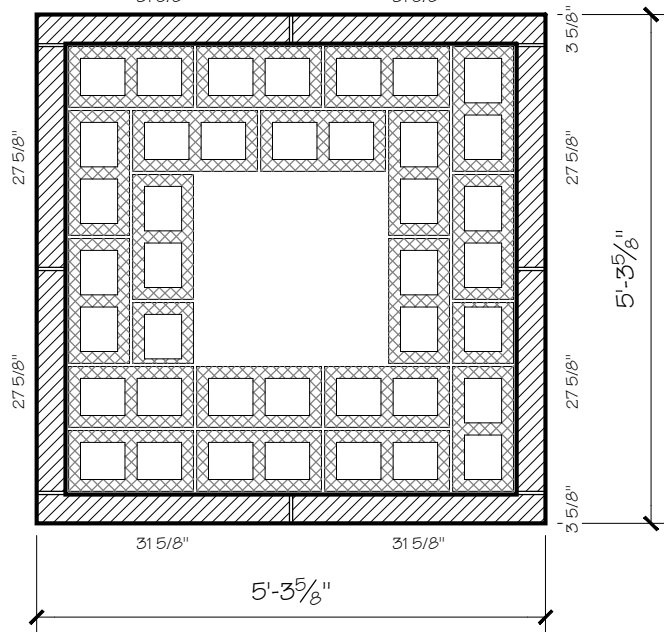
9 SECTION THRU COURSE PATTERN "C" 1/2" = 1'-0"
