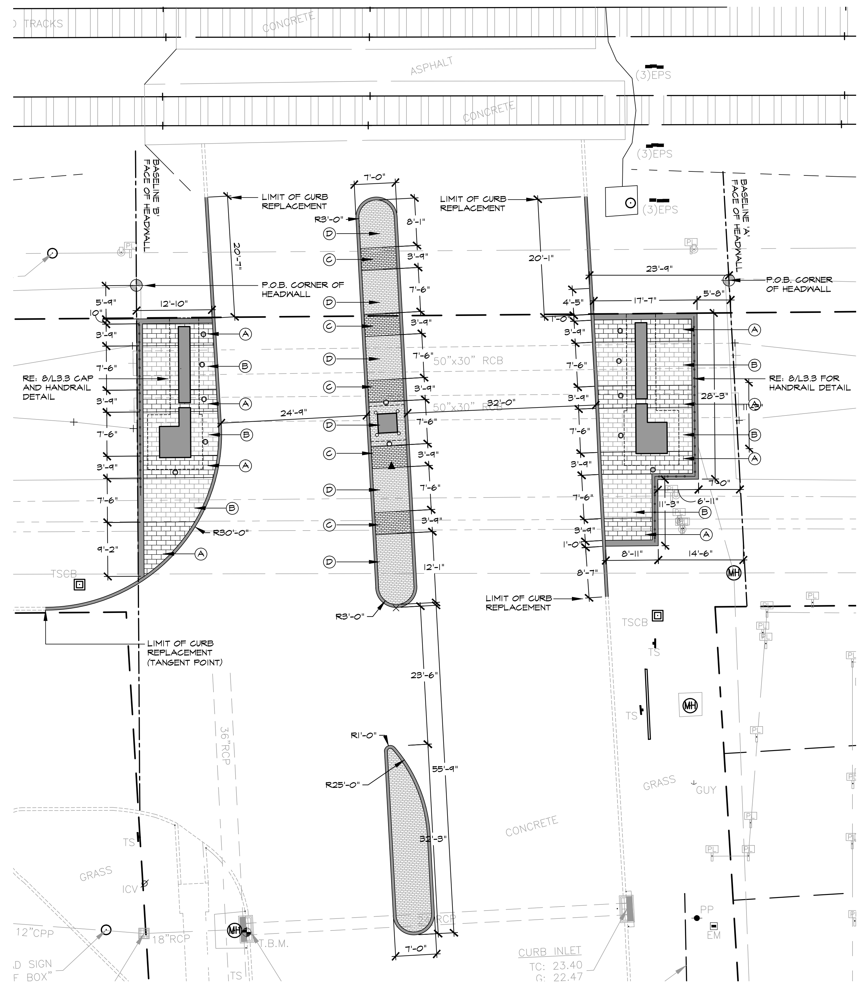
1 PAVING LAYOUT PLAN
