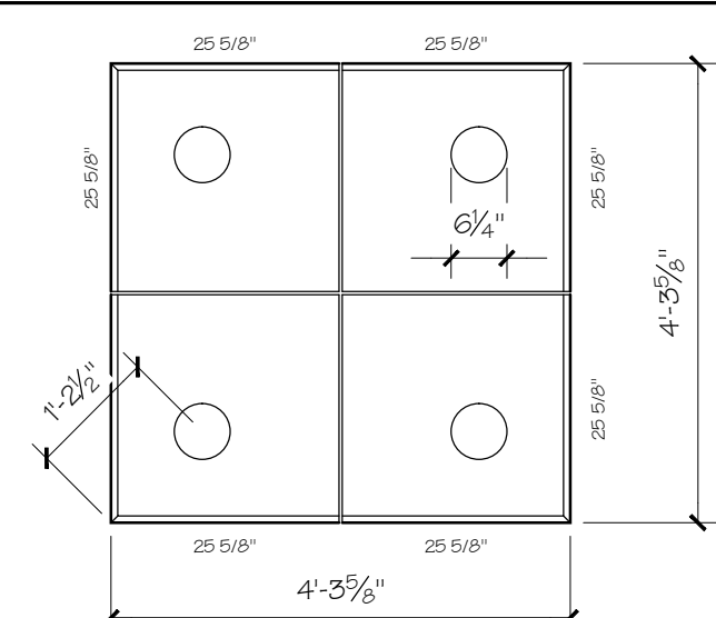
14 PLAN VIEW @ TOWER CAP 1/2" = 1'-0"
