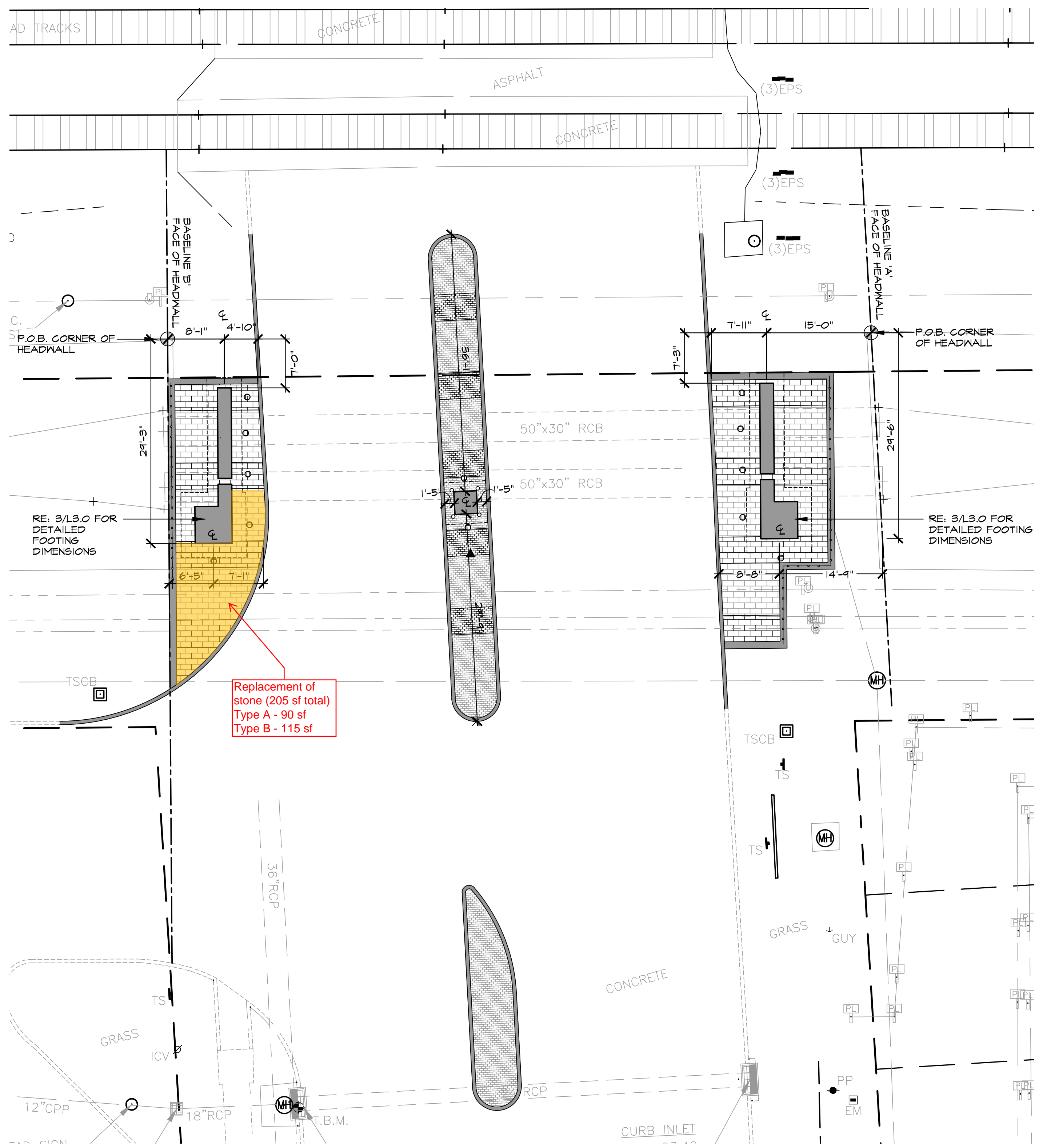
2 GATEWAY LAYOUT PLAN
