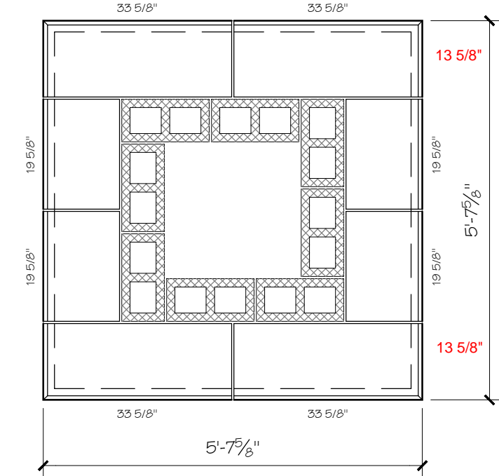
11 PLAN VIEW @ TOWER CAP 1/2" = 1'-0"
