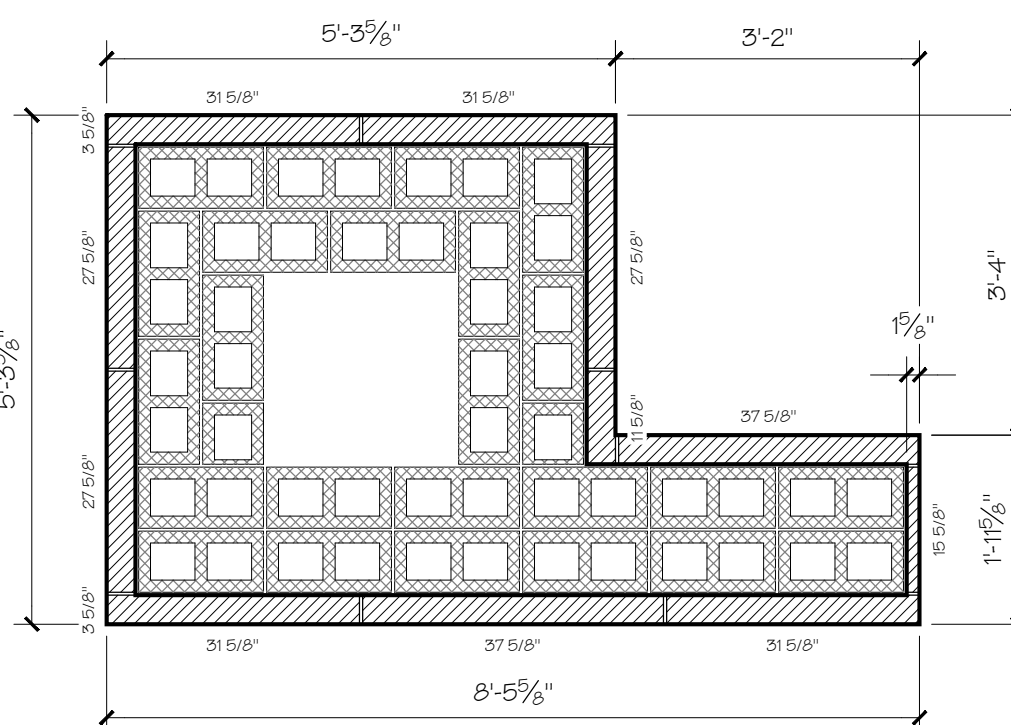
6 SECTION THRU COURSE PATTERN "A" 1/2" = 1'-0"
