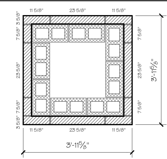
13 SECTION THRU COURSE PATTERN "F" 1/2" = 1'-0"
