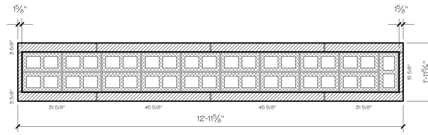
17 ELEVATION @ WALL 1/2" = 1'-0"
