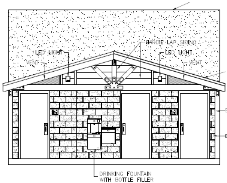
1 FRONT ELEVATION
